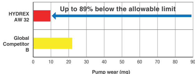
Eaton 35VQ25 Hydraulic Pump Wear Test *
