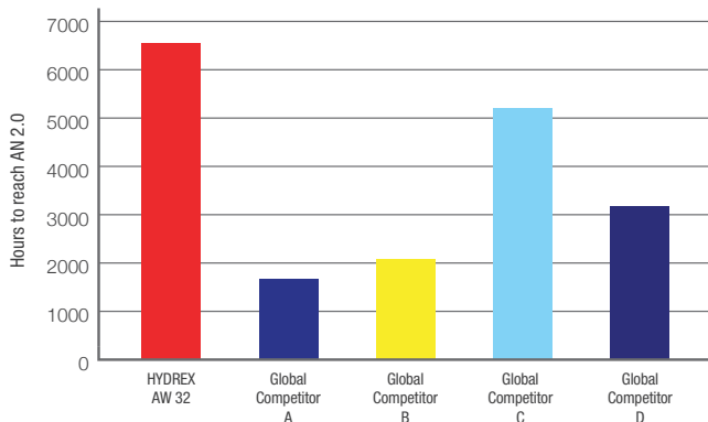
Oxidation Life Comparison ASTM D943 Test (ISO 32)
