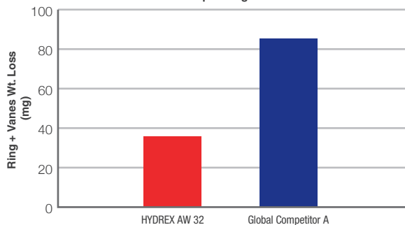
Modified Eaton 35VQ25 Hydraulic Pump Test
